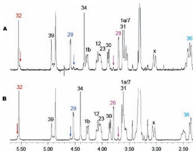
Figure 3. Partial 1 H NMR spectra (500 MHz, CD 3 OD) of the synthetic (34 S )-stereoisomer (panel A) and (34 R )-stereoisomer (panel B).
