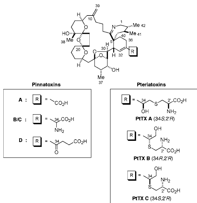
Figure 1. Structures of PnTXs and PtTXs.
